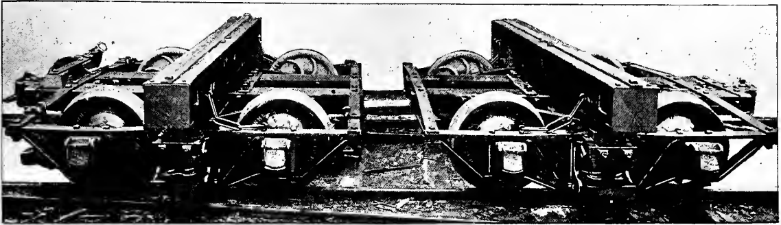
Fig. 36. LOGGING CAR, BUILT BY THE RUSSELL WHEEL & FOUNDRY COMPANY. Truck length, 8 ft. 4 ins. Height, 32 ins. Capacity, 50,000 lbs. Weight, 9,400 lbs. (Details are shown in Figs. 352-351.)
